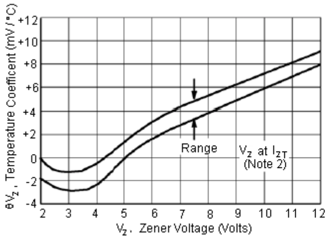
Temperature Coefficients (-55°C to +150°C temperature range; 90% of the units are in the ranges indicated.)
